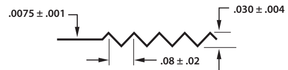
CORRUGATED SHIELD DETAILS
