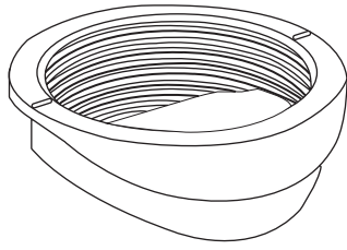
EPDM Rubber Gasket SIZES: 8" - 10", 12" - 15", 16" - 27" or 28" & larger profile
